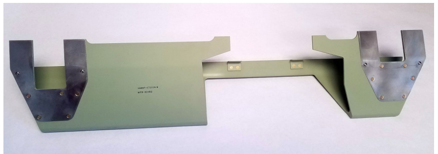
Machined Extrusion and Sheet Metal Assy Aluminum and Stainless Size: 18x8x3in
